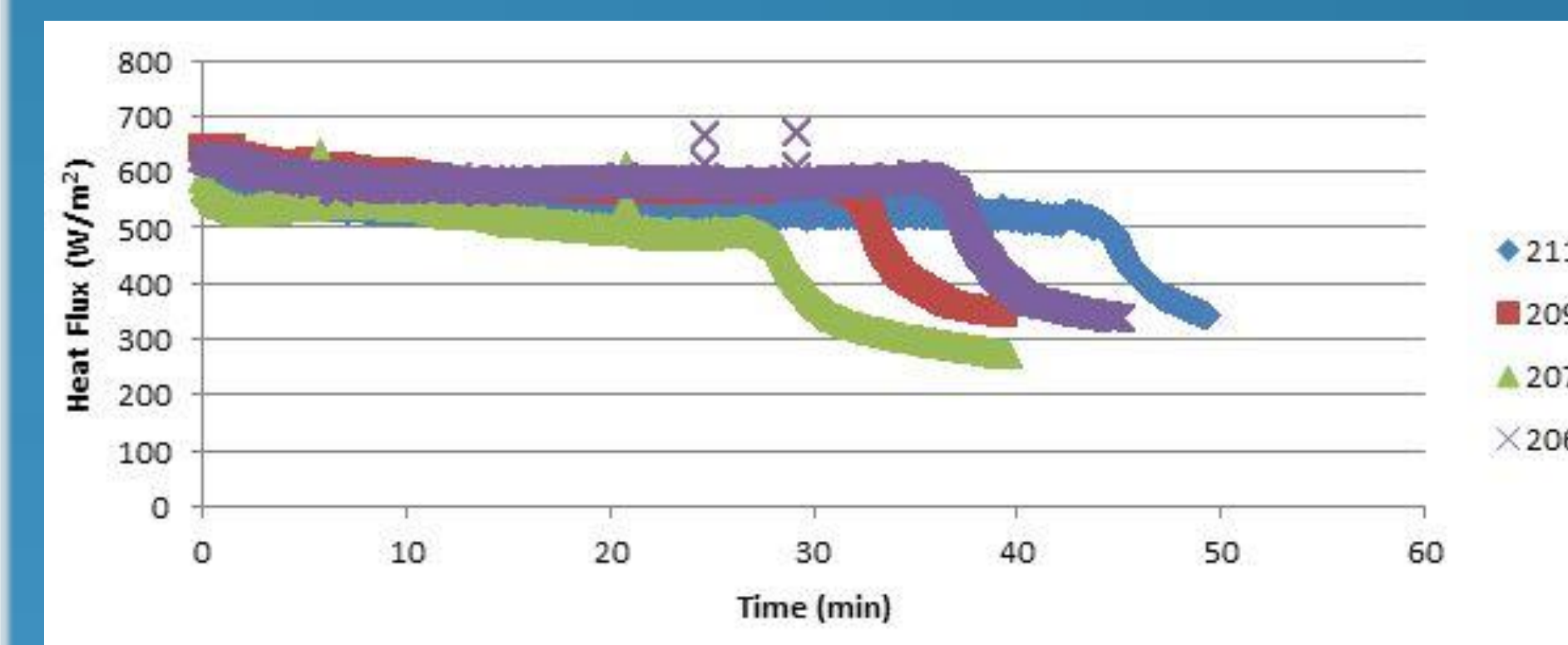
Figure 5. A composite heat flux-time graph from the boil off stage from the vapor and top outside thermocouples
