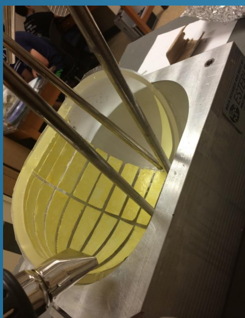
Figure 1. Construction of aerogel tank with stabilization apparatus and heat gun.
