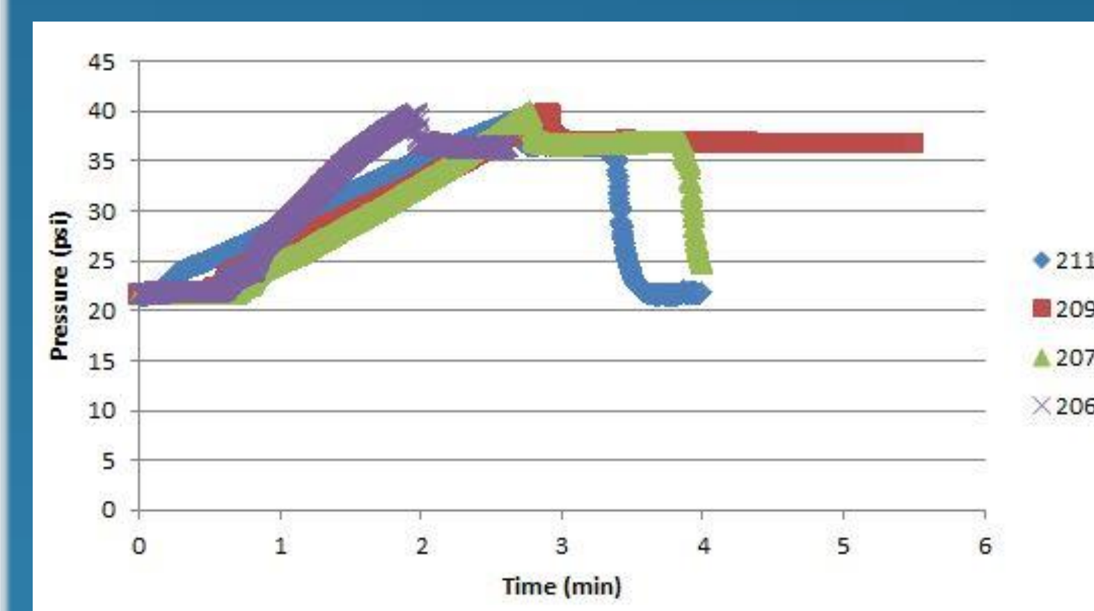
Figure 3. A composite pressure-time graph from the pressurization stage.
