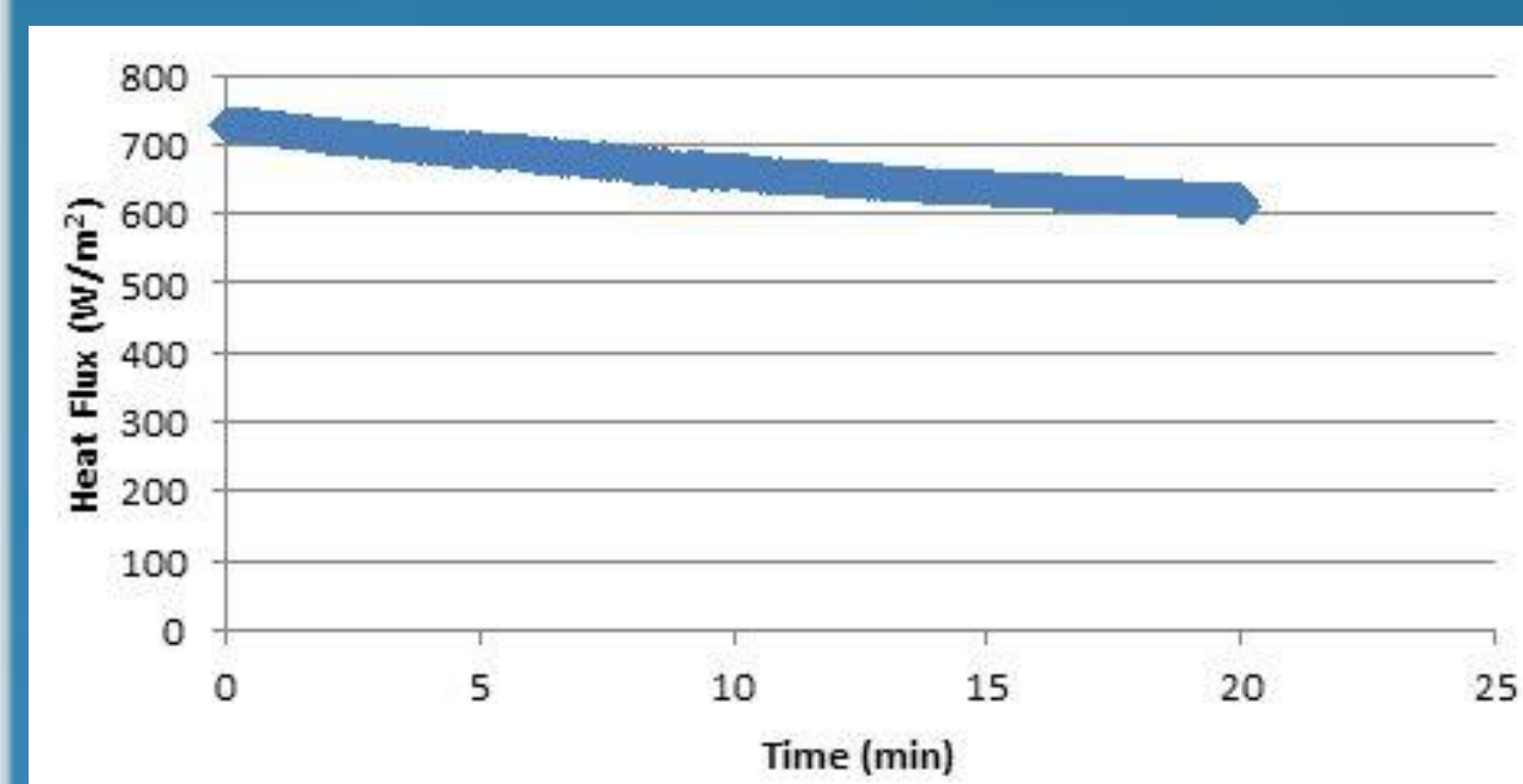
Figure 4. An averaged heat flux-time graph from the constant liquid phase from the vapor and top outside thermocouples.
