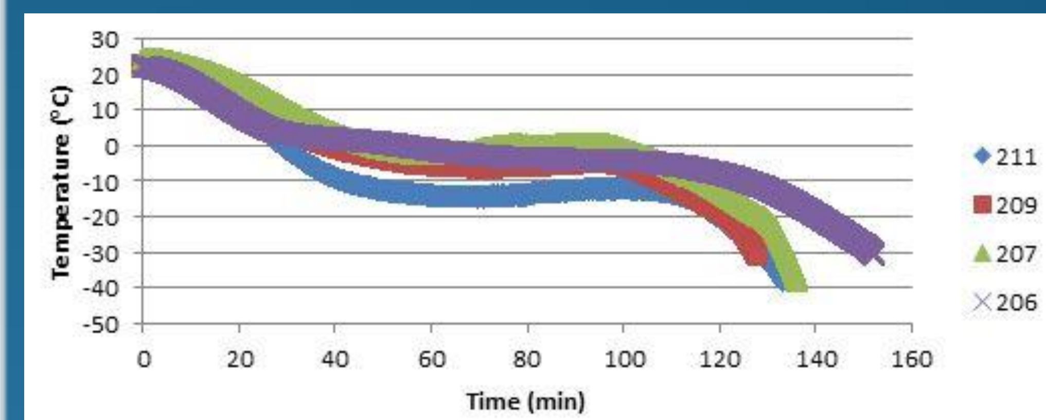
Figure 2. A composite temperature-time graph from the top outside thermocouple from the precool stage.
